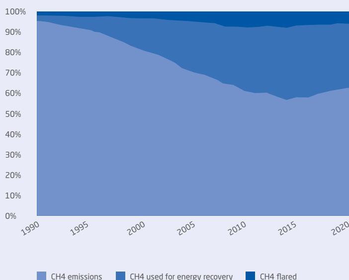
Figure 3: Evolution of the share of methane used for energy recovery, methane flared and CH4 emissions in managed landfills in the EU (EEA, 2022)
