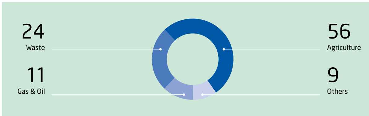
Figure 2: EU anthropogenic methane emission - 2021
